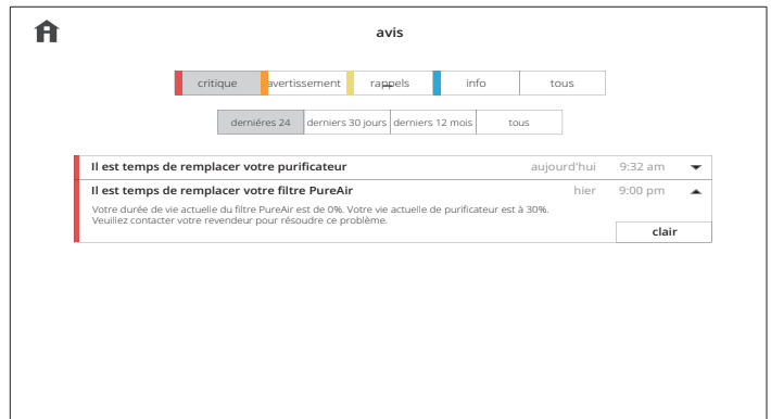
Figure 5. Notifications
