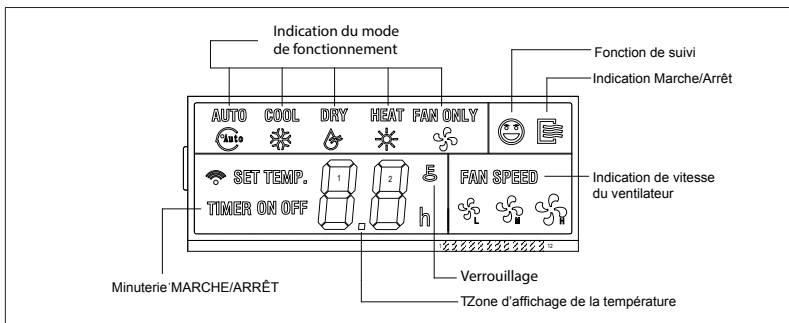
Figure 6. Display
