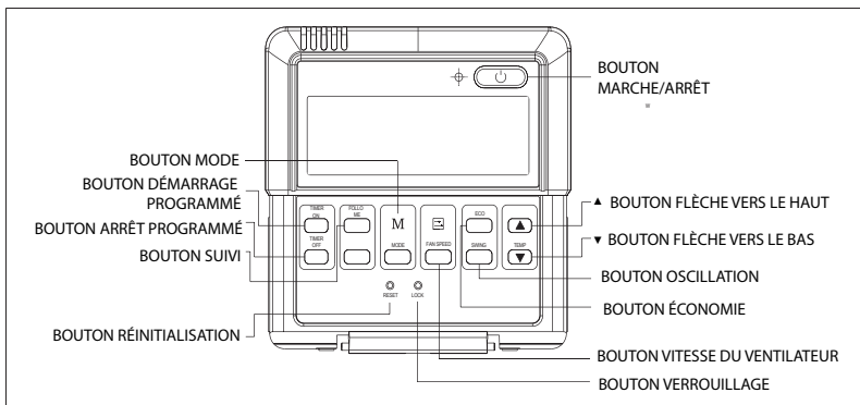
Figure 7. Buttons
